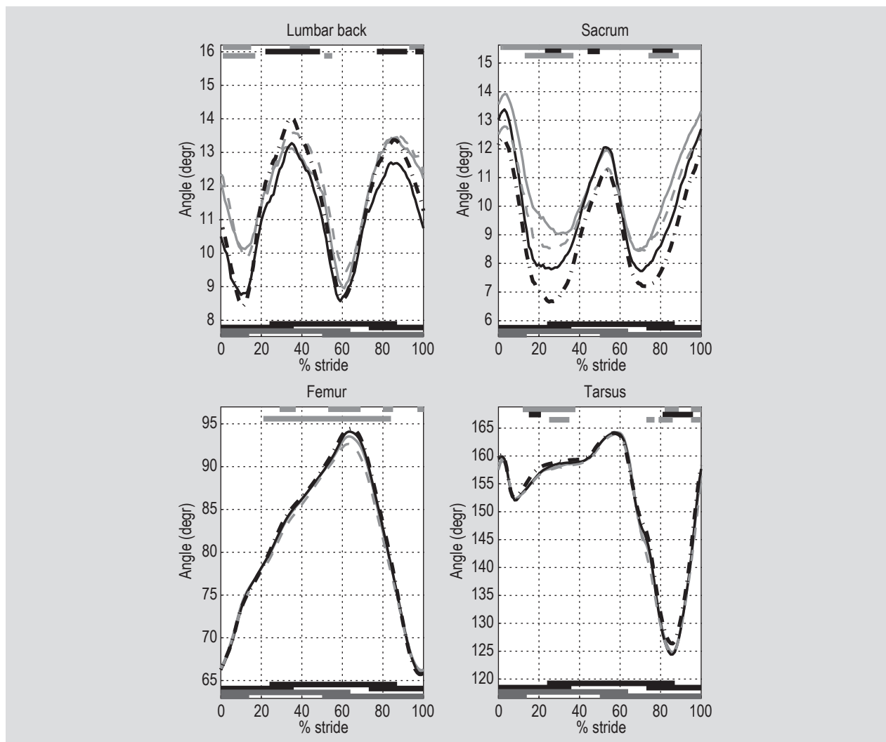
Figure 3. Group mean curves for selected variables with the stride normalised to 101 points, 0-100%, in horses ridden at walk with the head and neck in four different head and neck positions (HNP); HNP3 (solid grey line), HNP4 (solid black line), HNP5 (dashed grey line) and a mean of the speed-matched HNP2 (dash-dotted heavy black line). The horizontal bars at the top indicate significant differences ( P < 0.05 ) between a speed-matched measurement in the reference (competition) position HNP2 and HNP3 (upper grey bar), HNP4 (black bar) or HNP5 (lower grey bar). The horizontal bars at the bottom represent stance phases of (from top to bottom) the left and right forelimbs (black bars) and left and right hindlimbs (grey bars).
