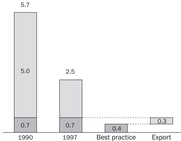
Figure 8. Evolution of water consumption in industrial ethanol production from sugarcane ( \text{m}^3/\text{ton} of sugarcane). Source: Dedini (2008).
