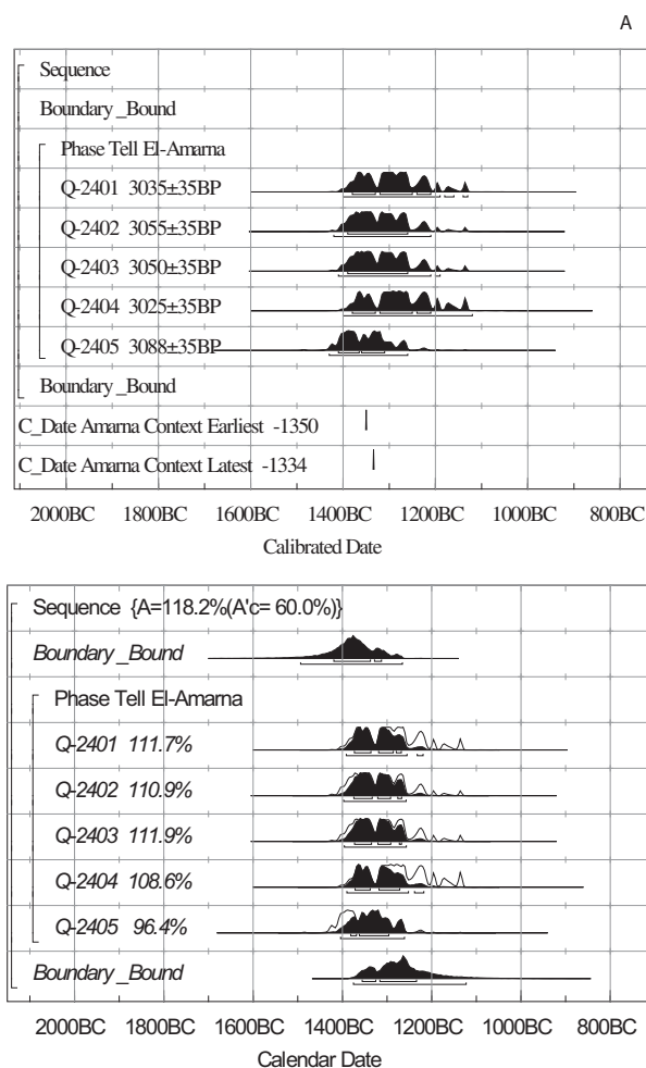
Figure III. 1.1.A. Calibrated calendar ages for the radiocarbon data reported from Tell el-Amarna, Egypt (Switsur, n. 41, 178–188) compared to the historical date for the context (see text). The upper and lower lines under each histogram indicate respectively the 1\sigma (68.2%) and 2\sigma (95.4%) calibrated age ranges. B. Sequence analysis (solid histograms) of the Amarna data (with the individual probabilities from A. indicated by the hollow histograms) as a phase within calculated boundaries. The Amarna data are entirely consistent with the historical age estimate for the context. Calibration and analysis employing OxCal 3.9 (Bronk Ramsey, n. 35 and later versions, with curve resolution set at 4) and INTCAL98 (n. 15). Q-2401, wood; Q-2402, charcoal; Q-2403, skin; Q-2404, horn; Q-2505, bone. Weighted average of all five data: 3050±16 BP (1), weighted average of just the three definitely shorter-lived samples 3054±20 BP (2). 2\sigma (95.4%) confidence calibrated ranges respectively (1) 1388–1331 BC (46.6%), 1322–1260 BC (48.8%), and (2) 1393–1260 BC (94%), 1228–1222 BC (1.4%).
