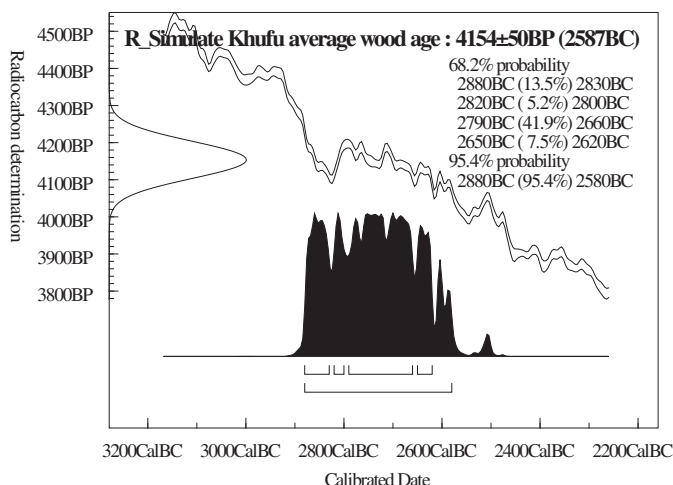
Figure III. 1.3. Simulated radiocarbon age for a calendar date of 2587 \pm 50 BC using OxCal 3.9 (Bronk Ramsey, n. 35 and later versions with curve resolution set at 4) and INTCAL98 (n. 15). Note: every simulation run produces a slightly different outcome—this is a ‘typical’ output based on a number of runs. This simulated calendar age is an example of possible typical age of ‘average’ wood from a monument built in the reign of Cheops (reign starts 2604/2593/2554/2551 BC and ends 2581/2570/2531/2528 BC: Beckerath, Chronologie ; Kitchen n. 43; Baines & Málek, n. 60), given a typical +50 \pm 50 year ‘old wood’ adjustment. The calibrated radiocarbon age intersects with the c.2900–2500 BC plateau in the radiocarbon calibration curve, and offers several 1\sigma ranges within a large 2\sigma range c.2880–2580 BC. We thus see as a function of the natural history of radiocarbon fluctuations that real dates in the early 26th century BC yield calibrated radiocarbon ranges mainly apparently too early, with the real date just creeping into the last few years of the calibrated age range. It is noteworthy that the average radiocarbon age from the 45 samples used for the Pyramid of Cheops at Giza is in fact 4147 \pm 10 BP (Bonani et al. , n. 50, 1315)—almost exactly the 4154BP radiocarbon age derived by the simulation of a calendar date of 2587 \pm 50 BC, as shown above. Thus it appears that the Cheops data do, on average, yield a plausible age for wood used in his reign (with this average wood typically +50 or so years in age, give or take a range, versus the actual use date—and the large range within the Cheops data, see below, indicates such a range, or more, in the real wood ages, apart from any contaminating factors from associated mortar/limestone). Because of the history of radiocarbon variations (the 2900–2500 BC plateau), only the very last part of the calibrated range indicates the real age. These data, and the other similar OK data in Bonani et al. (n. 50) where the ‘real’ age at best creeps into the end of the calibrated age range, or lies shortly afterwards, therefore do not provide evidence of any additional offset beyond old wood and the calibration outcomes given the history of natural radiocarbon levels c.2900–2500 BC. They provide no evidence at all for claims of hypothetical 100–300 years too early offsets in Mediterranean radiocarbon ages based on claims of putative upwelling of old carbon (Keenan) 67 —something for which there is no positive evidence within an order of magnitude (Manning et al. 2002, n. 33).
