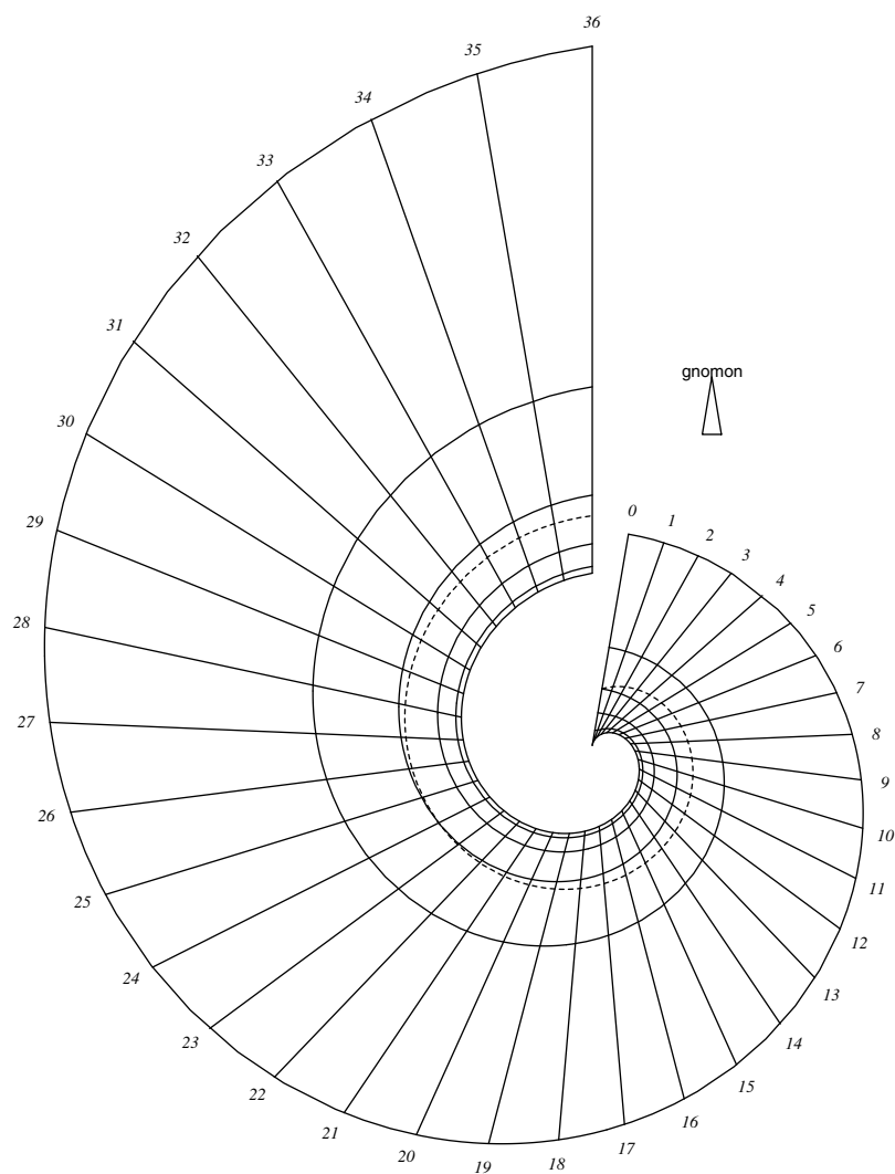
FIG. 3.34. al-Marrākushī's ḥalazūn in terms of the midday shadow (the outermost curve is for the first hour, the innermost one for midday, the dashed one for the ʿaṣr )
