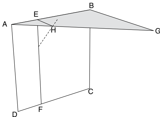
FIG. 3.45. Principle of the universal 'aşr' dials
