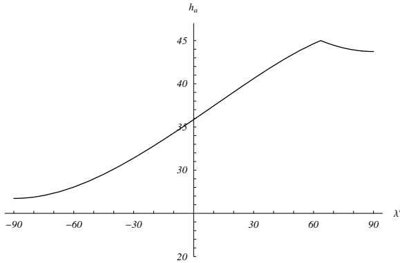
FIG. 3.42. Plot of h_a(\lambda') for \phi = 21^\circ
