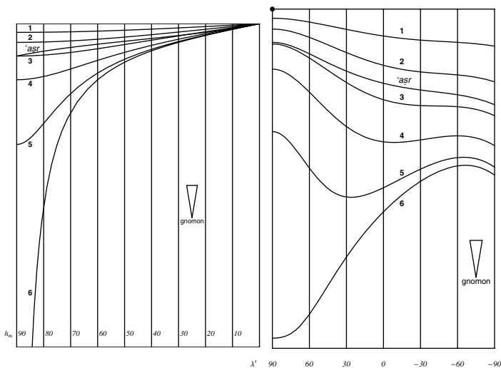
FIG. 3.23. Universal “locust’s leg”, with meridian altitude scale
