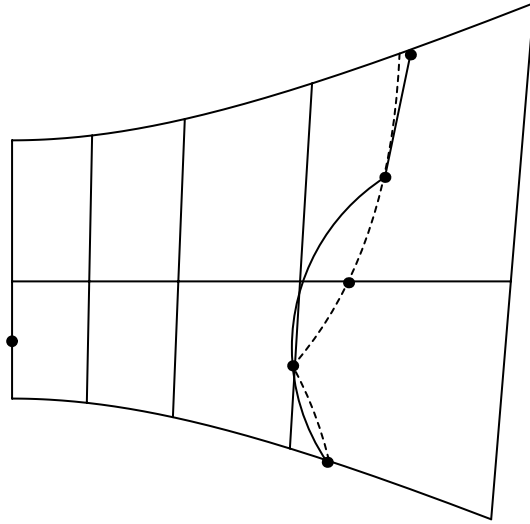
FIG. 3.44. Najm al-Dīn's unsuccessful 'aṣr curve for latitude 12^\circ (the accurate one is dashed)
