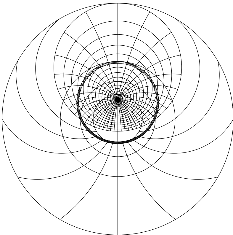
FIG. 2.3. The kāmil astrolabe (with accurate seasonal hour-lines)
