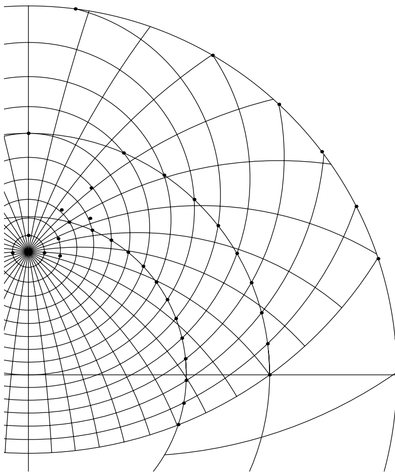
FIG. 2.1. Representation of the entries of Table T.1 for constructing the altitude circles (note that the three entries for Taurus and Gemini are clearly in error)
