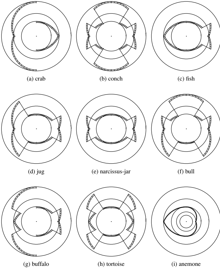
FIG. 2.6. al-Sijzi's and al-Biruni's mixed retes
