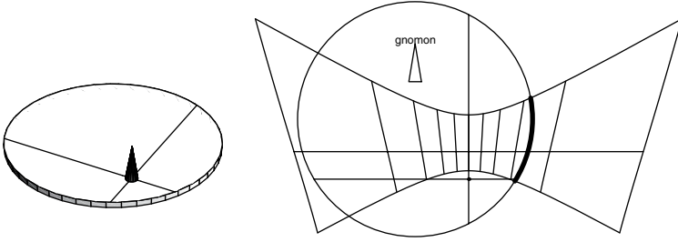
FIG. 3.40. Circle for finding the ʿaṣr FIG. 3.41. Representation thereof over a horizontal sundial
