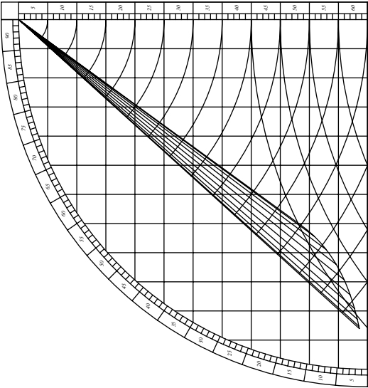
FIG. 5.12. Najm al-Dīn's mujamam quadrant
