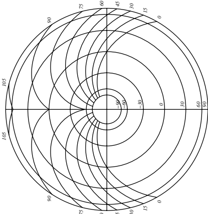
(b) Interpretation of the second version of Ch. 84
