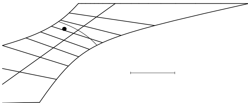
FIG. 4.8. An inclined sundial (with D = -45^\circ , i = 30^\circ ) displaying equal hours before sunset, as illustrated in Ch. 115
