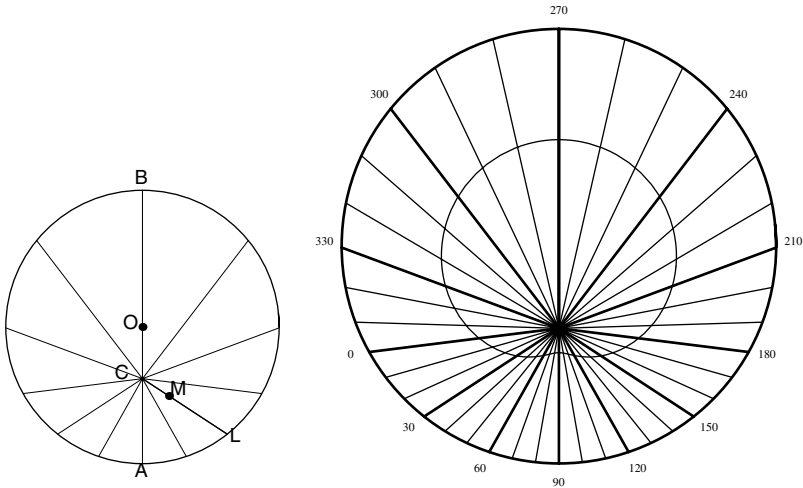
FIG. 3.32. Construction procedure in Ch. 88
