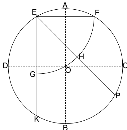
FIG. 3.20. Construction of the ring dial
