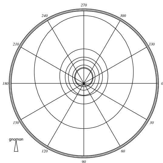
FIG. 3.27. al-Šūfī's 'lemon' dial
