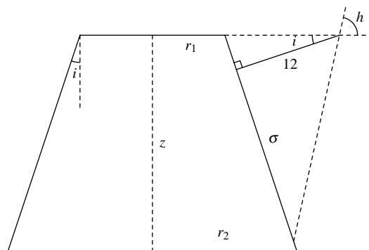
FIG. 3.25. Principle of the conical dial
