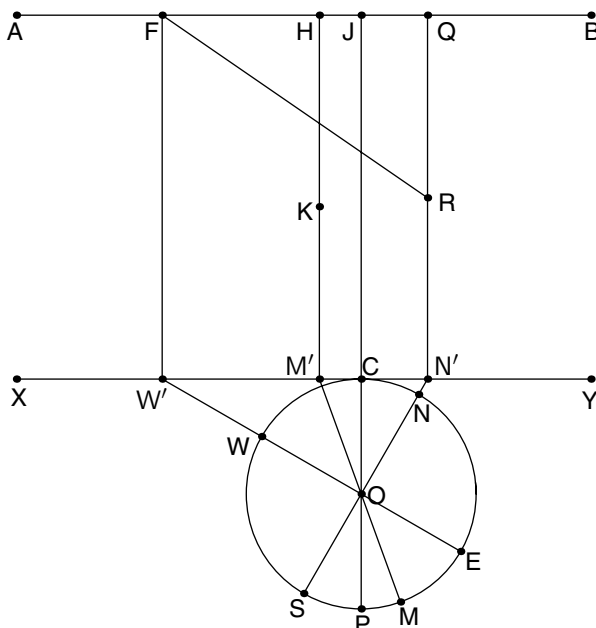
FIG. 4.4. Construction of a declining vertical sundial
