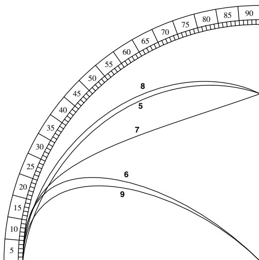
FIG. 3.50. Further possibilities of representing the 'aṣr on a sine quadrant
