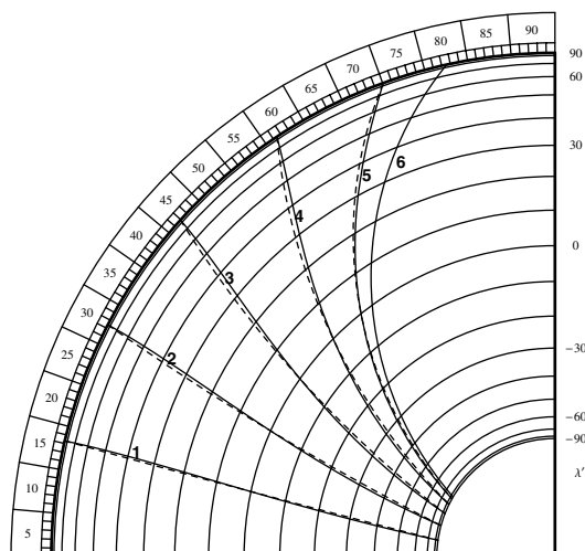
FIG. 3.4. The horary quadrant with “circles of equation”
