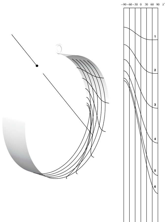
FIG. 3.21. Najm al-Dīn's ring dial
