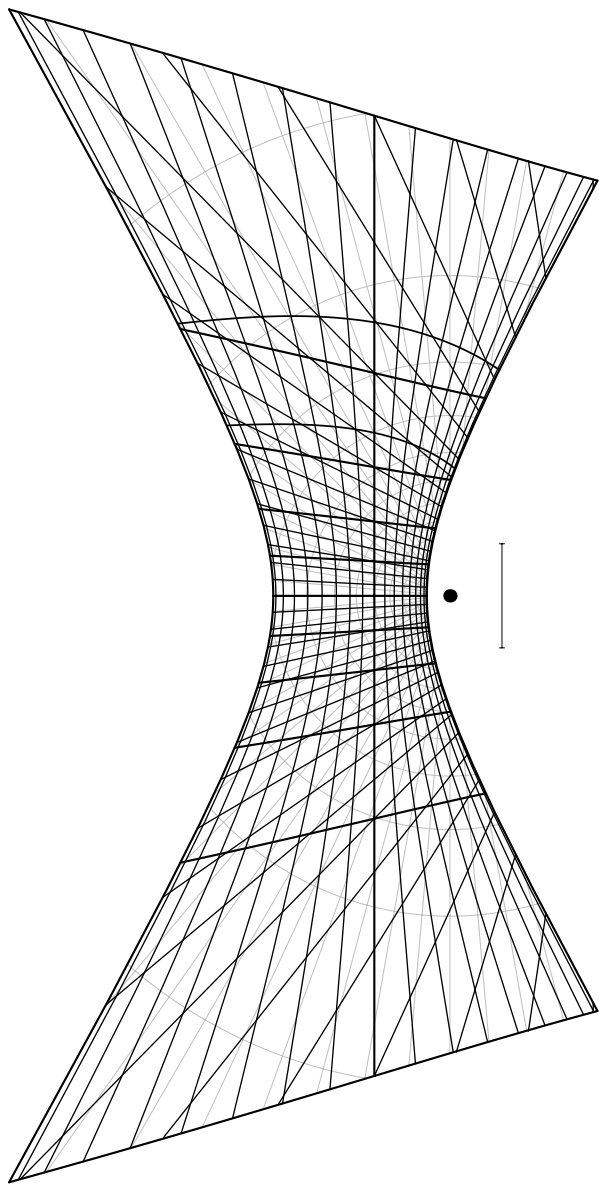
FIG. 4.1. Najm al-Dīn's complex horizontal sundial
