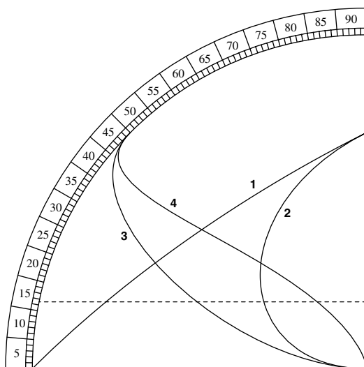
FIG. 3.49. Najm al-Dīn's 'aṣr curves on a sine quadrant
