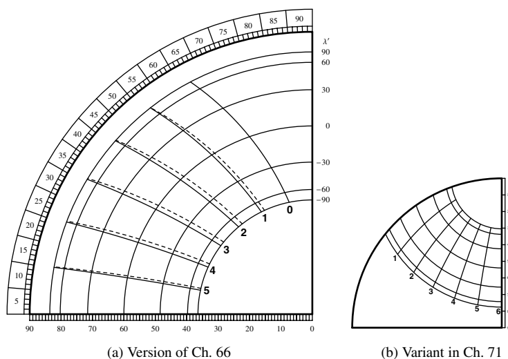
FIG. 3.15. Horary quadrants with (almost) equidistant hour-lines
