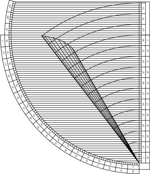
FIG. 5.11. al-Marrākushī's "figure for finding the hour-angle"
