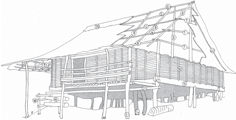
Figure 2.1. Outline structure of the Nuaulu house, showing relative position of selected components mentioned in the text.
